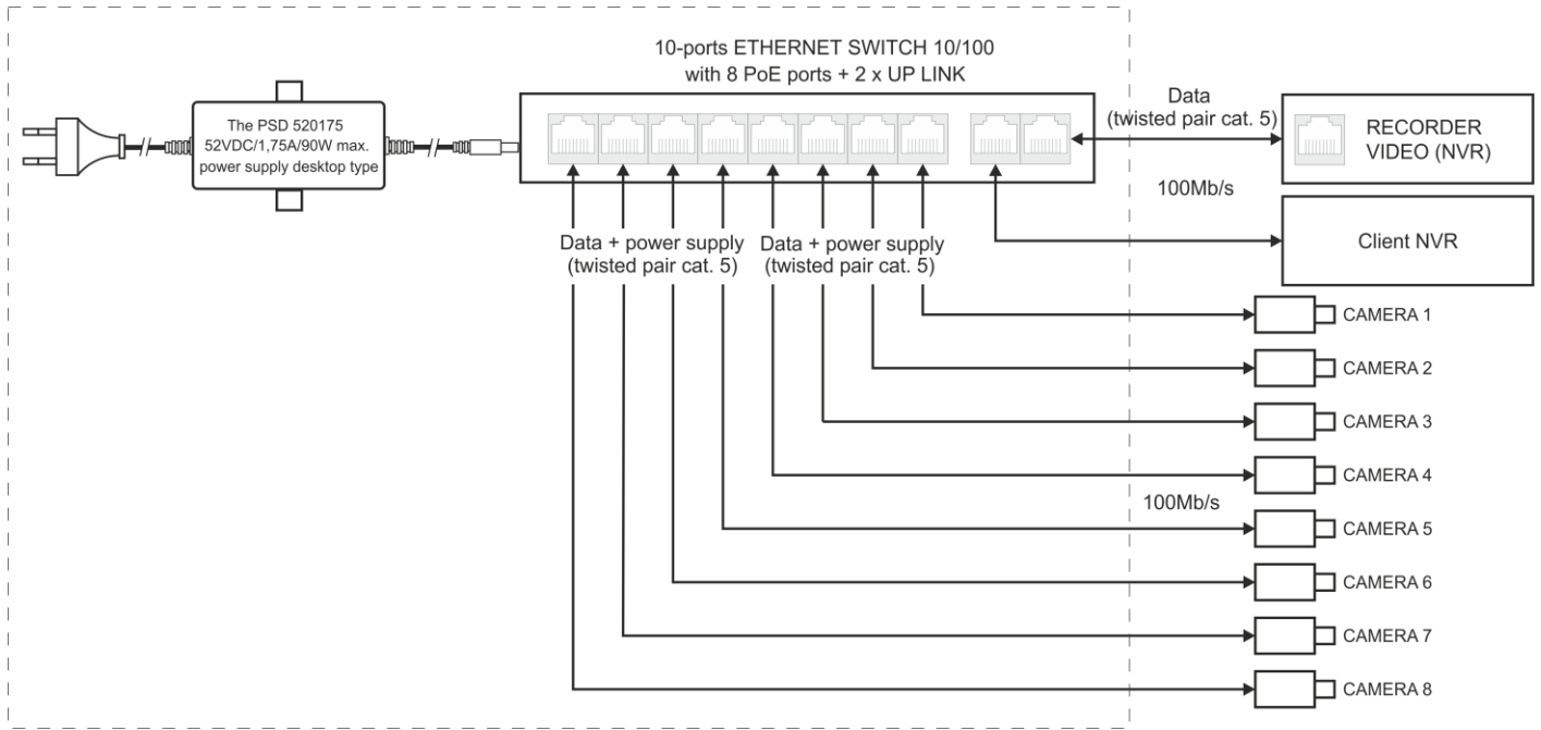
Fig. 1. Block diagram.
